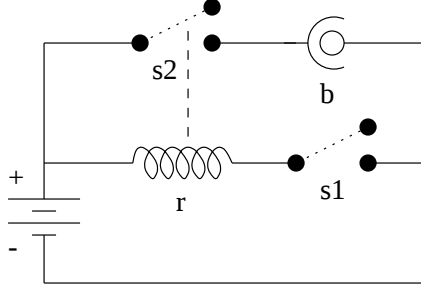
Figure 6.1: Circuit \mathcal{AC}_{diag}
